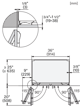
KFMC3642FD, KFMC3844FD, MasterCool III, panel ready, Draufsicht (Skizze)
