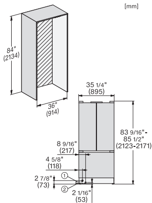
KFMC3642FD, KFMC3844FD, MasterCool III, Installation, panel ready (*Fußnote) (Skizze)
