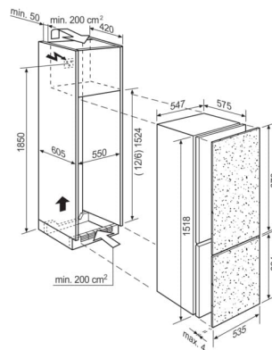
EK276BN / EK274BN
